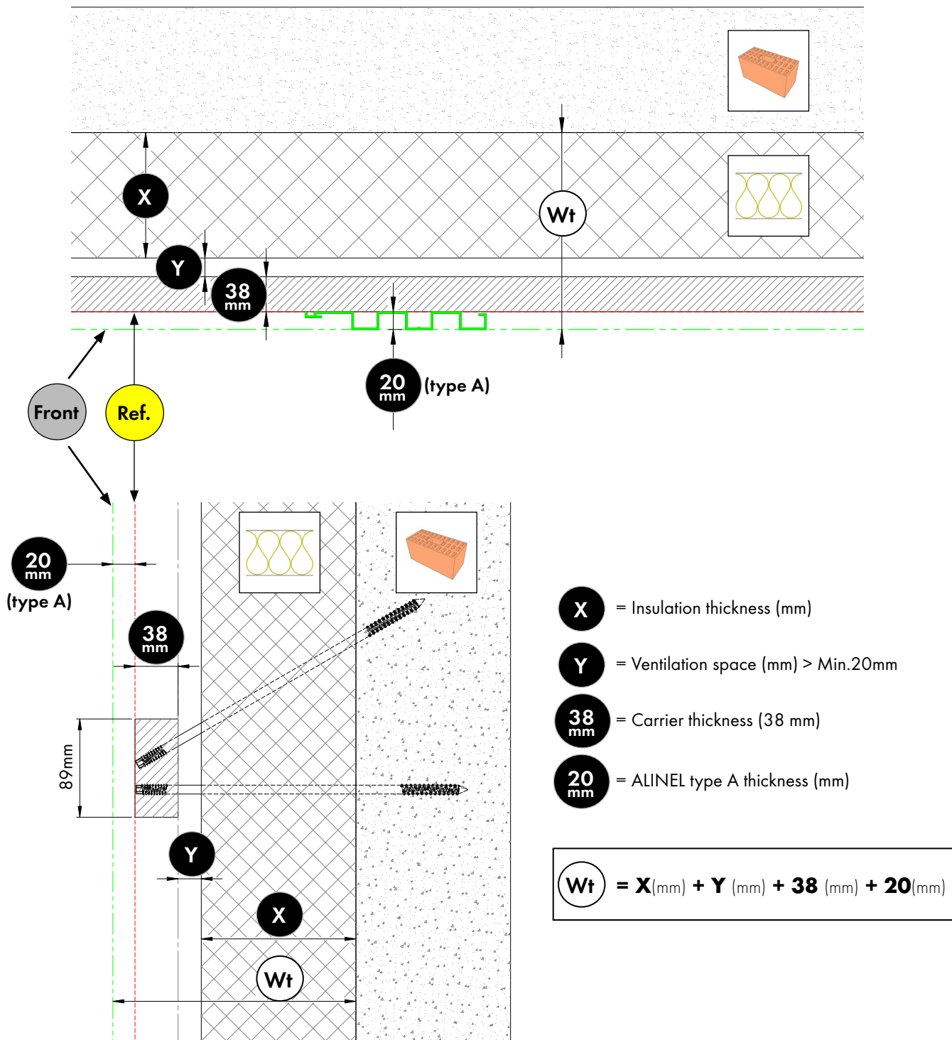
Verticale doorsnede / Section verticale / Verticalschnitt / Vertical section
